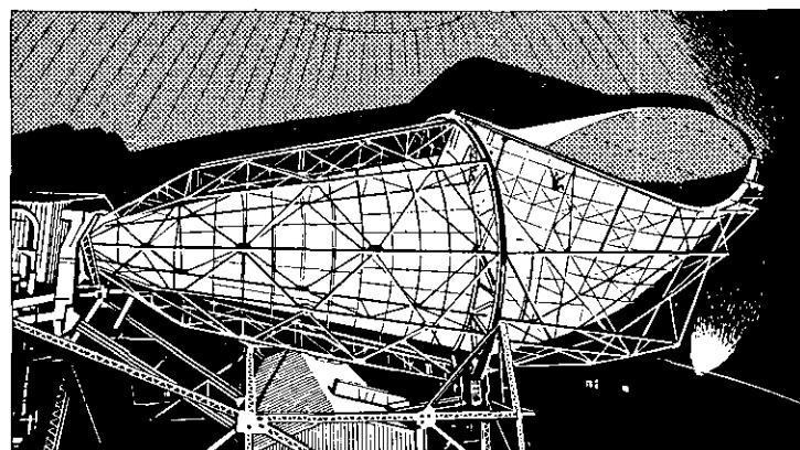
INSIDE GROUND STATION "RADOME" AT ANDOVER, MAINE. Giant antenna (note man near rim of horn) concentrates signals to Telstar in a narrow, powerful beam. In the same antenna a receiver amplifies signals coming from Telstar ten billion times.
